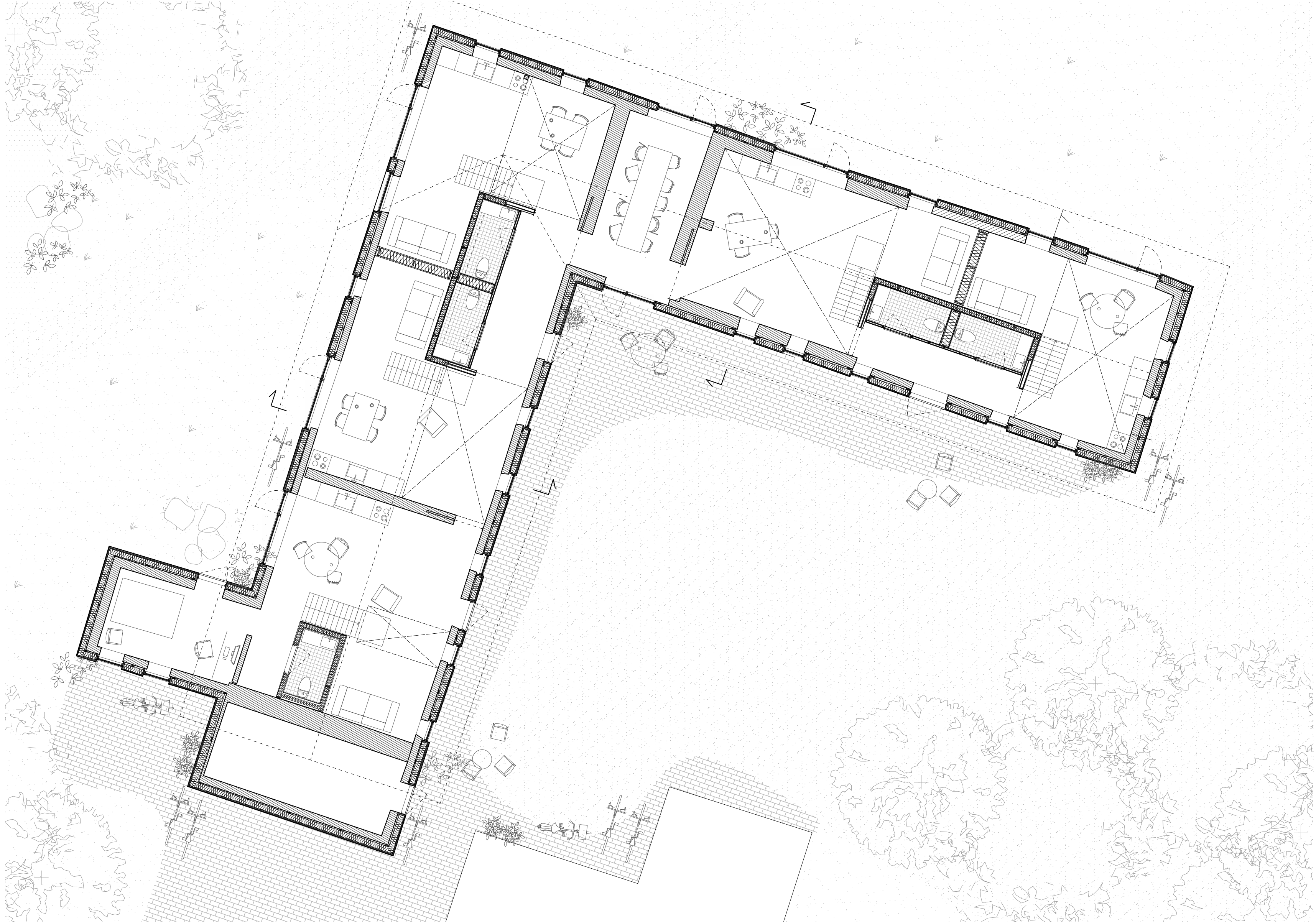
Plan, stueetage
